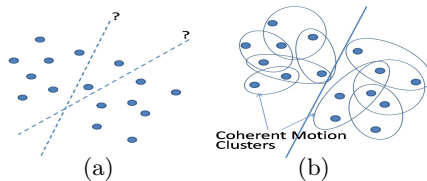
Figure 6. (a) Directly segmenting semantic regions according to the particles’ local features. (b) Segmenting semantic regions with the guidance of coherent motion clusters.
