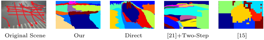
Figure 9. Constructed semantic regions of different methods. (Best viewed in color)
