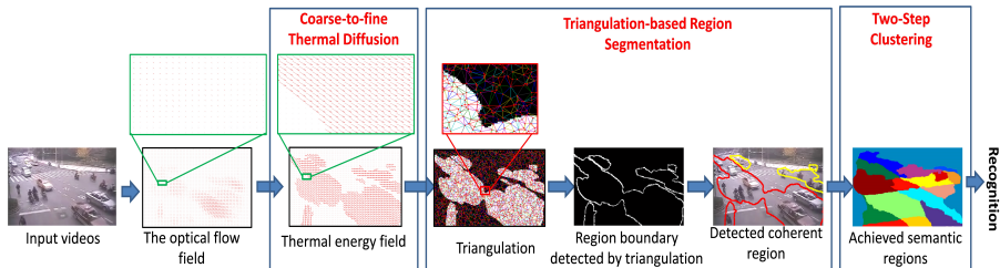
Figure 2. The flowchart of the proposed approach (best viewed in color).
