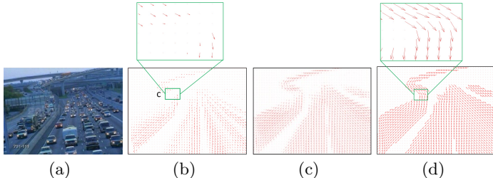
Figure 4. (a),(b): An input video frame and its input motion vector field; (c),(d): TEF results of Algorithm 1 after 1 and 3 iterations, respectively ( T_{max}=5 and T_{step}=1 ).
