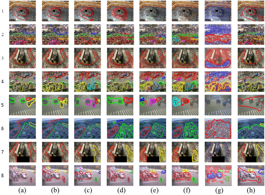
Figure 7. Coherent motion extraction results. (a): Ground Truth, (b): Results of our approach, (c): Results of [2], (d): Results of [21], (e): Results of [26], (f): Results of [27], (g): Results of [4], (h): Results of [22]. (Best viewed in color)
