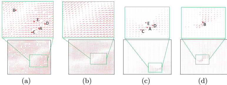
Figure 3. (a),(b): One input optical flow field and its thermal energy field; (c), (d): Individual thermal diffusion result by diffusing from a single heat source particle A and B to the entire field.
