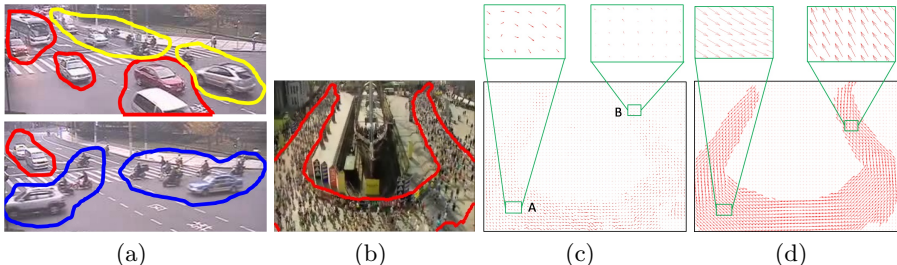
Figure 1. (a) Example time-varying coherent motions; (b) Example frame of a Marathon video sequence, the red curve is the ground truth coherent motion region; (c) Input motion vector field of (b); (d) Coherent motion field from (c) using the proposed approach (Best viewed in color).
